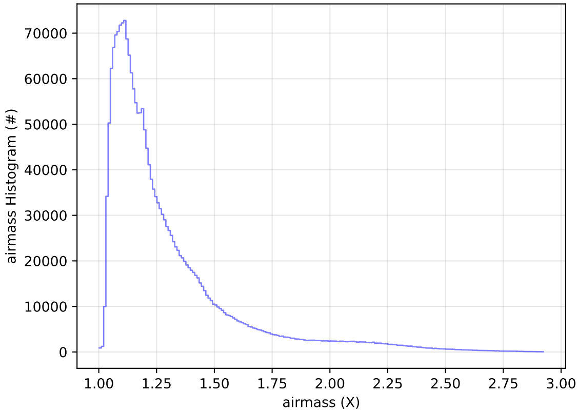
internal_u_expt27_nscale1.5v3.4_10yrs All sky all bands: airmass Histogram
