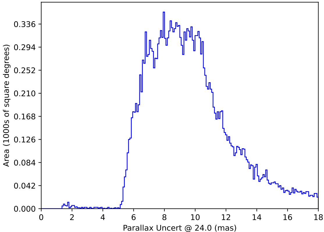
internal_u_expt27_nscale1.5v3.4_10yrs All sky: Parallax Uncert @ 24.0
