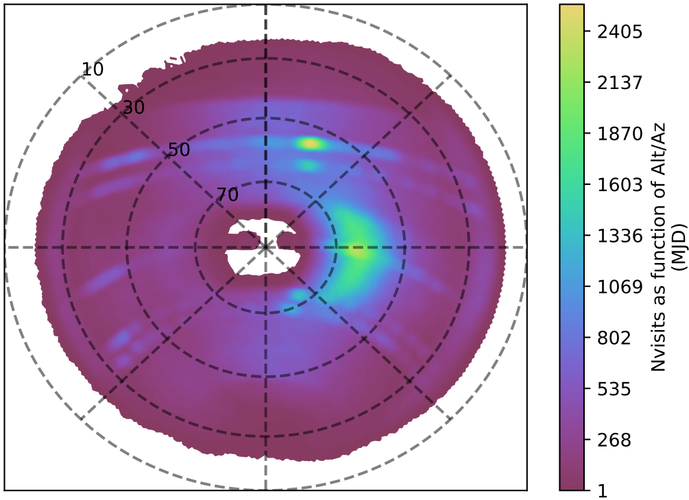
internal_u_expt27_nscale1.5v3.4_10yrs z band: Nvisits as function of Alt/Az
