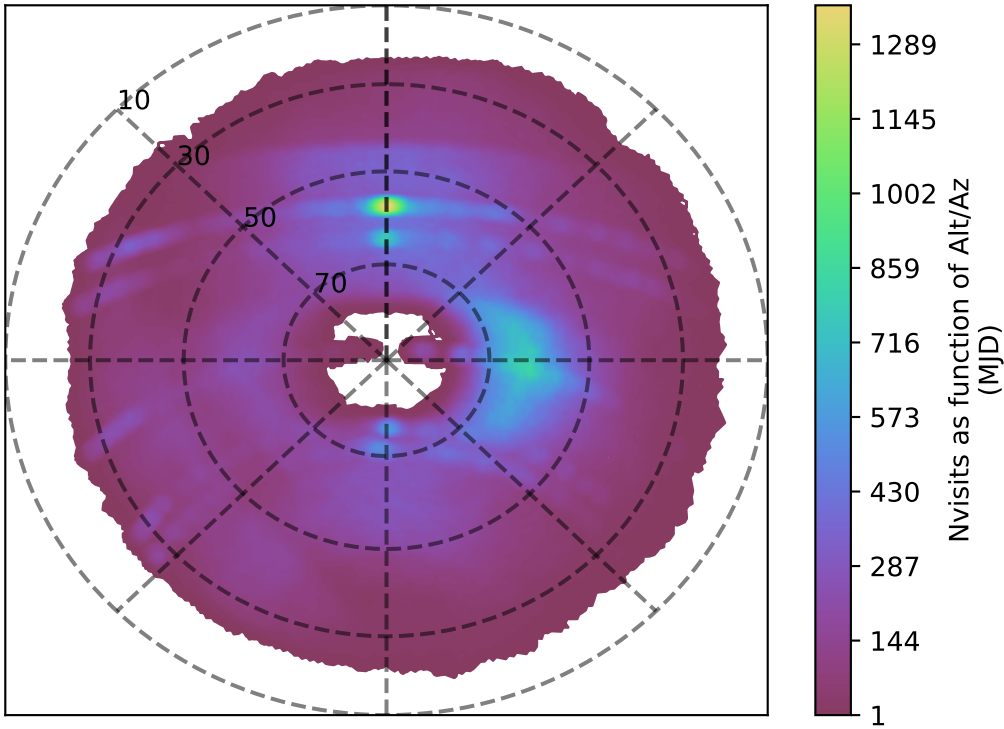
internal_u_expt27_nscale1.5v3.4_10yrs g band: Nvisits as function of Alt/Az
