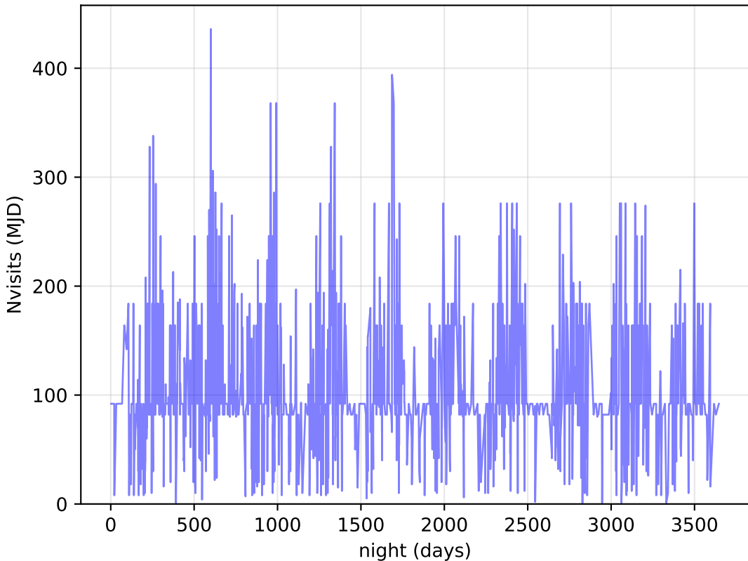
internal_u_expt27_nscale1.5v3.4_10yrs DDF: Nvisits
