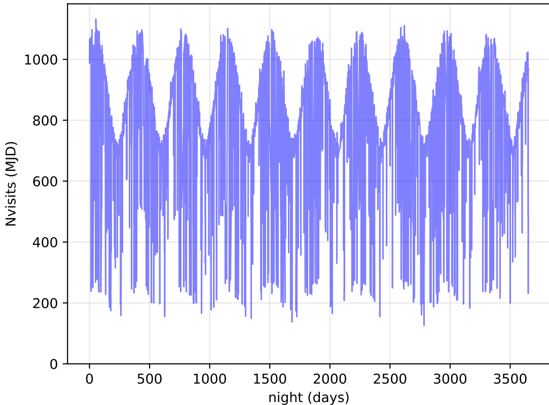
internal_u_expt27_nscale1.5v3.4_10yrs All visits: Nvisits
