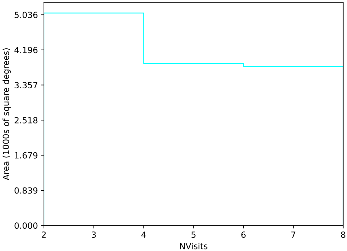
internal_u_expt27_nscale1.5v3.4_10yrs Yr 3-4 u band: NVisits
