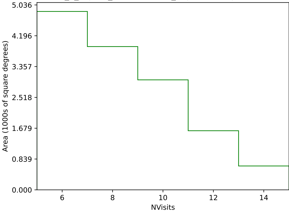
internal_u_expt27_nscale1.5v3.4_10yrs Yr 3-4 g band: NVisits
