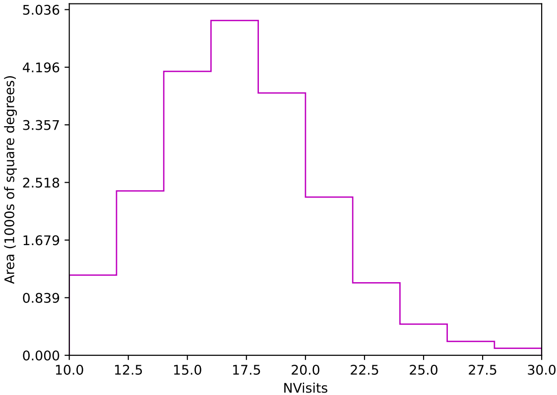
internal_u_expt27_nscale1.5v3.4_10yrs Yr 1 z band: NVisits
