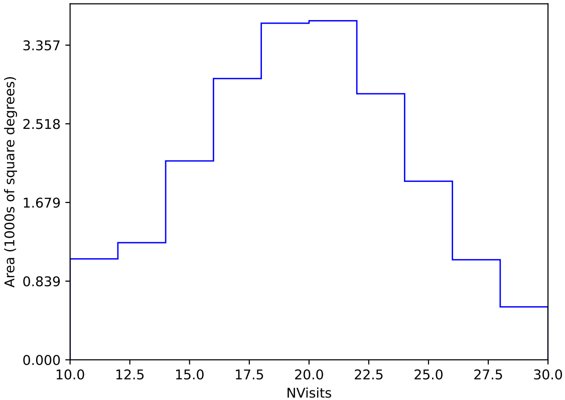
internal_u_expt27_nscale1.5v3.4_10yrs Yr 1 y band: NVisits
