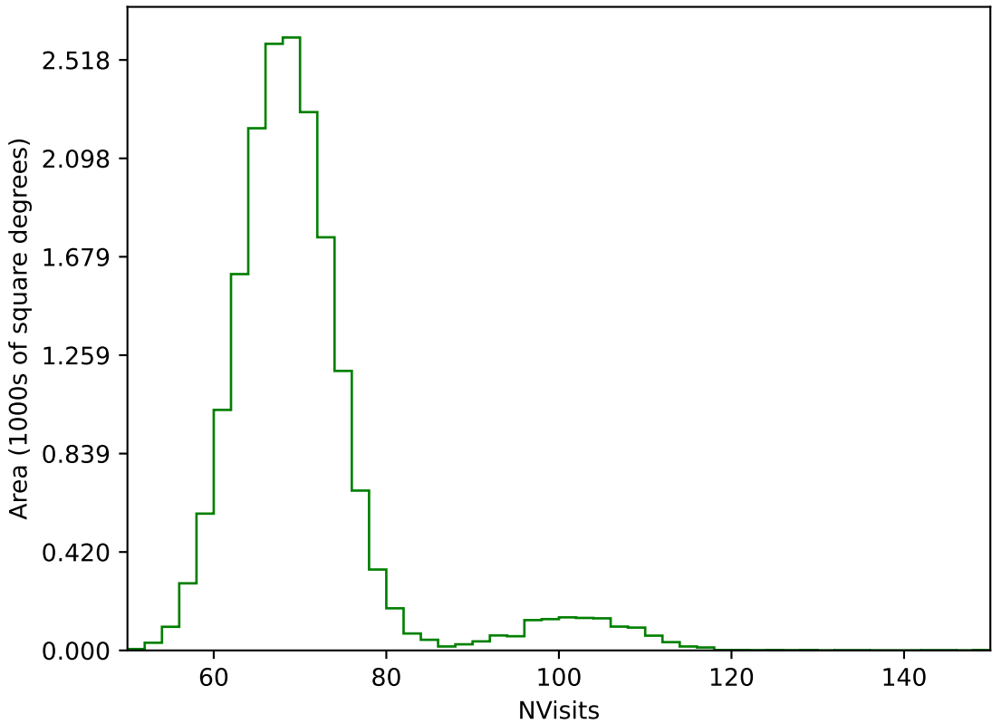
internal_u_expt27_nscale1.5v3.4_10yrs WFD g band: NVisits
