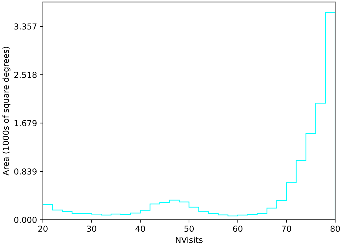
internal_u_expt27_nscale1.5v3.4_10yrs All sky u band: NVisits
