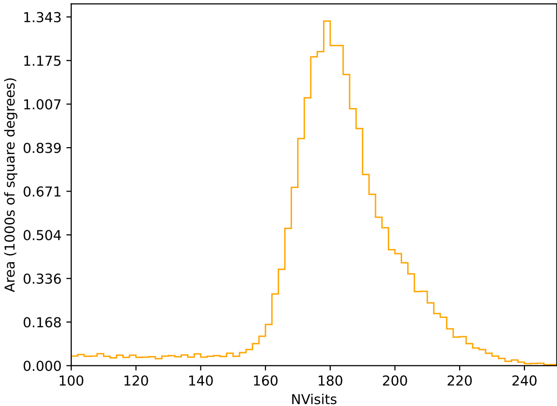
internal_u_expt27_nscale1.5v3.4_10yrs All sky r band: NVisits
