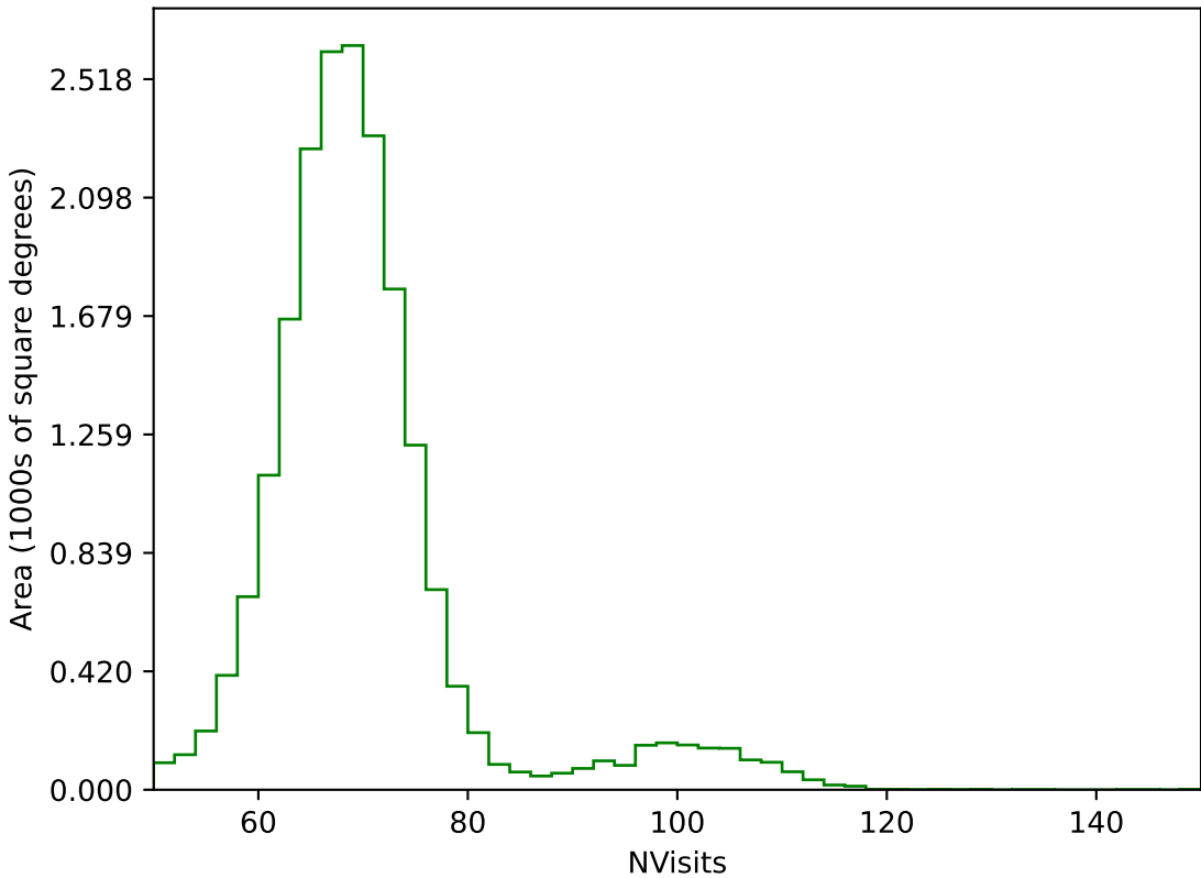
internal_u_expt27_nscale1.5v3.4_10yrs All sky g band: NVisits
