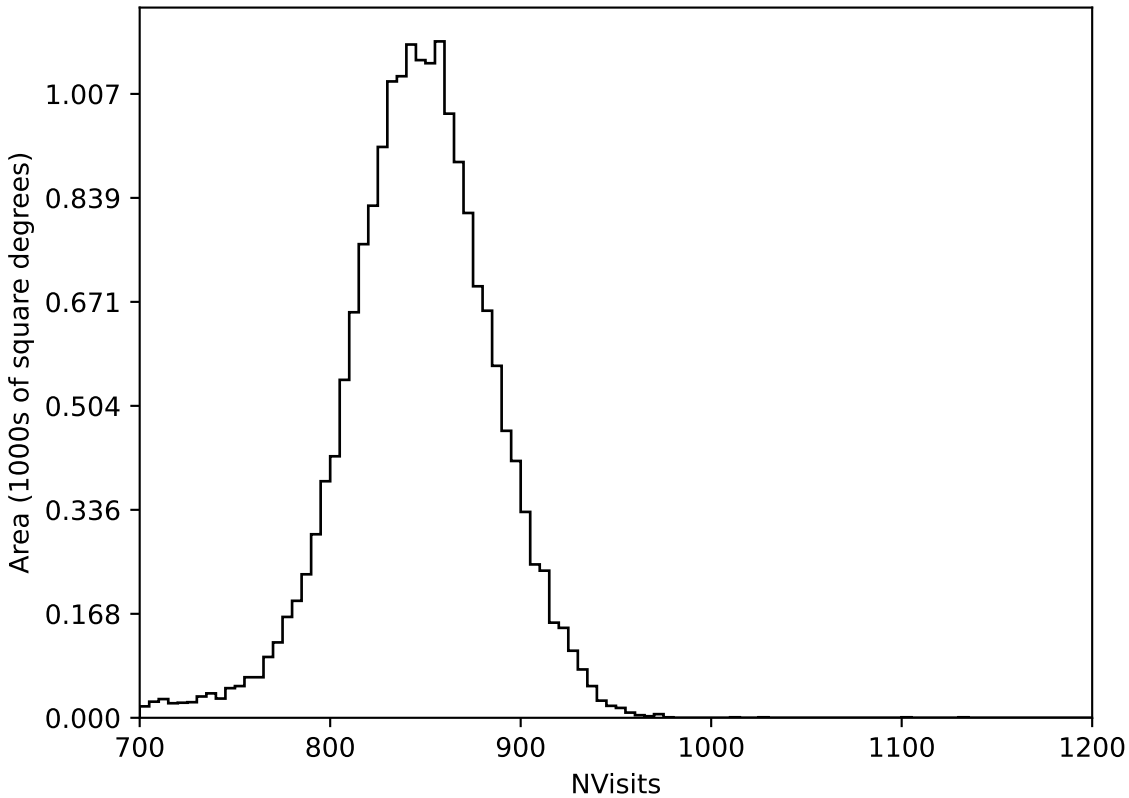
internal_u_expt27_nscale1.5v3.4_10yrs All sky all bands: NVisits
