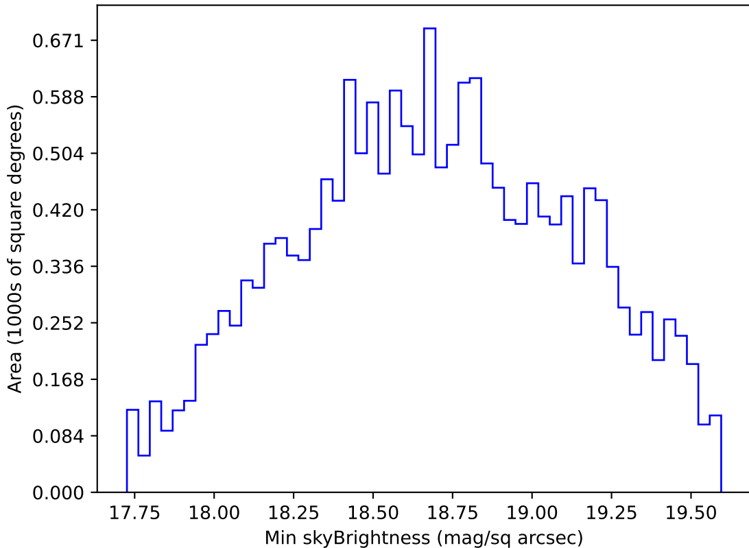
internal_u_expt27_nscale1.5v3.4_10yrs WFD r band: Min skyBrightness
