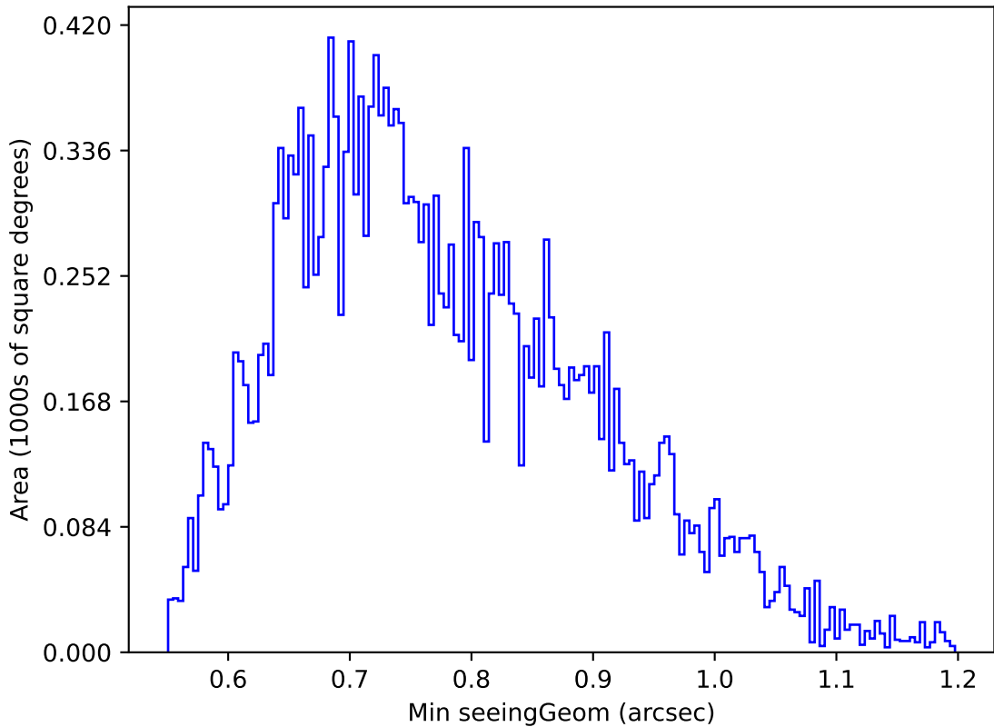
internal_u_expt27_nscale1.5v3.4_10yrs Yr 1 u band: Min seeingGeom
