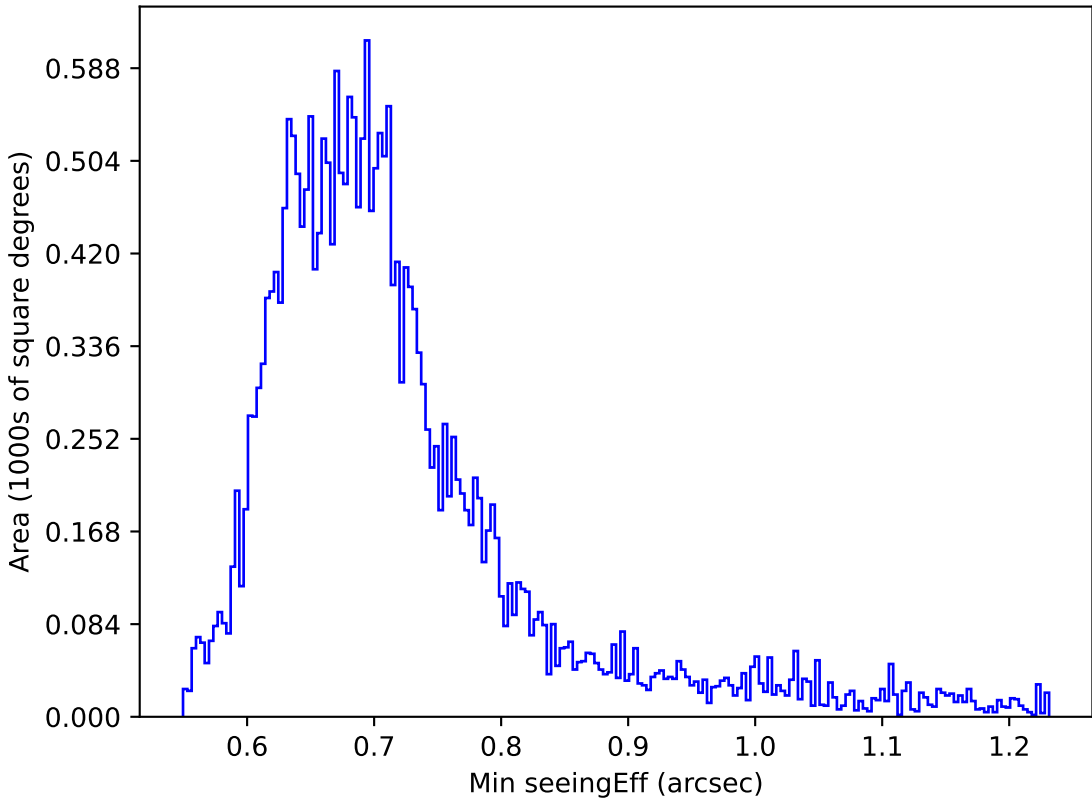
internal_u_expt27_nscale1.5v3.4_10yrs Yr 1 z band: Min seeingEff
