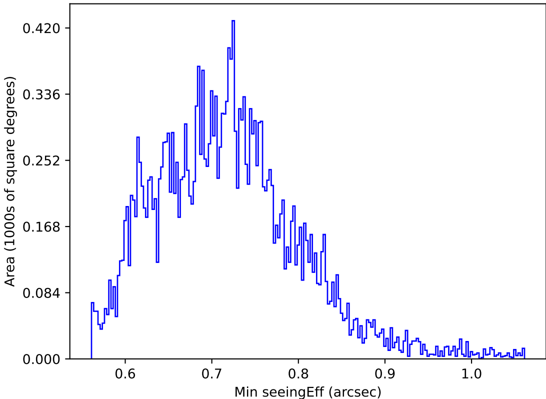
internal_u_expt27_nscale1.5v3.4_10yrs Yr 1 y band: Min seeingEff
