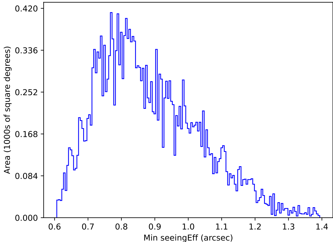
internal_u_expt27_nscale1.5v3.4_10yrs Yr 1 u band: Min seeingEff
