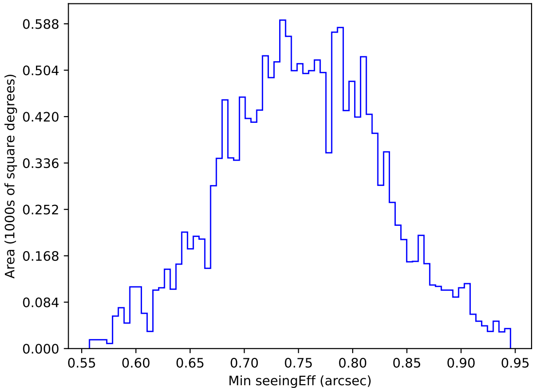
internal_u_expt27_nscale1.5v3.4_10yrs WFD u band: Min seeingEff
