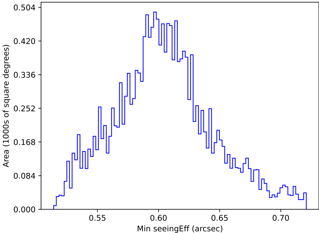
internal_u_expt27_nscale1.5v3.4_10yrs WFD i band: Min seeingEff
