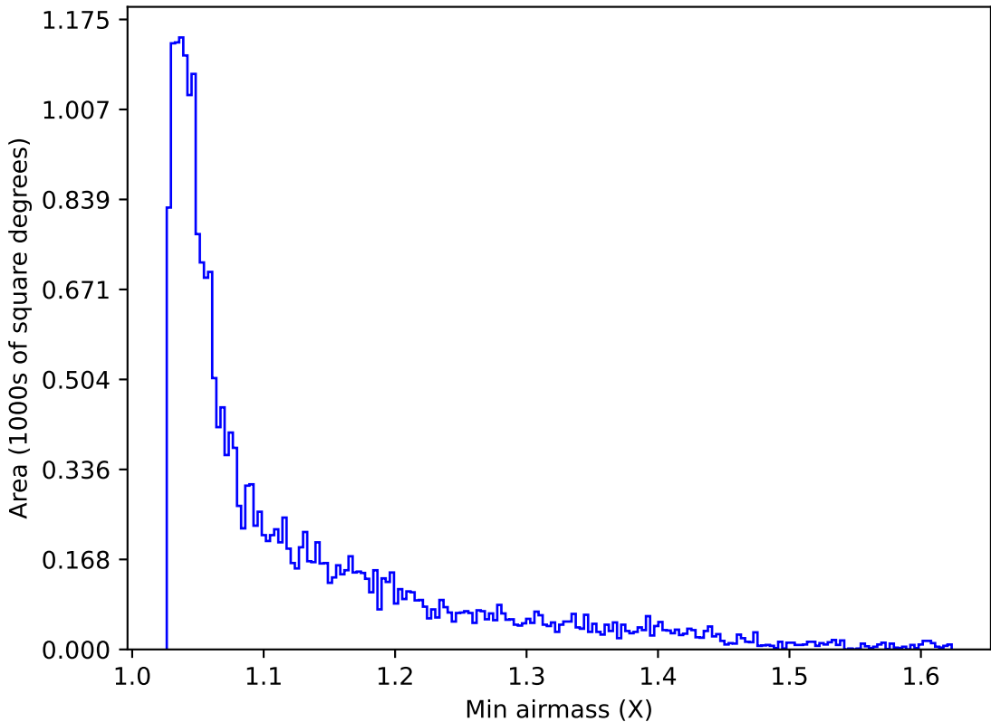
internal_u_expt27_nscale1.5v3.4_10yrs Yr 1 y band: Min airmass
