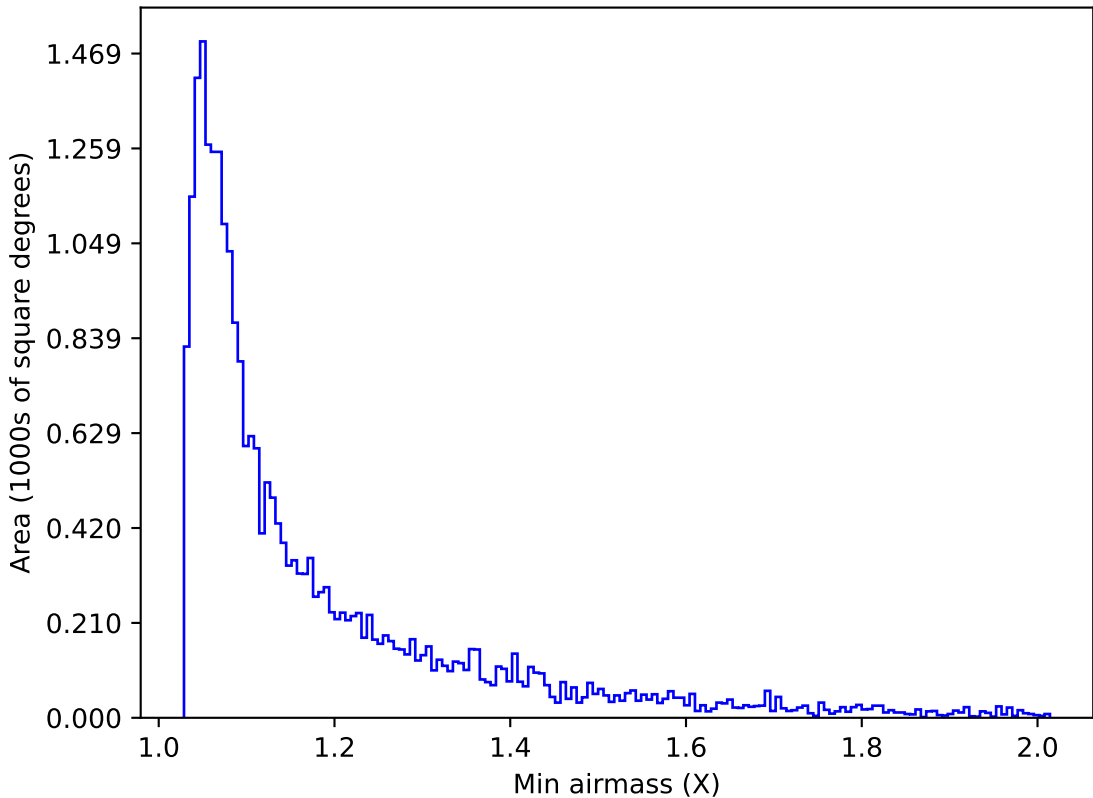
internal_u_expt27_nscale1.5v3.4_10yrs Yr 1 g band: Min airmass
