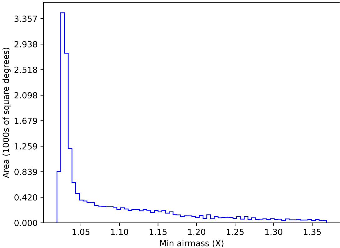
internal_u_expt27_nscale1.5v3.4_10yrs WFD z band: Min airmass
