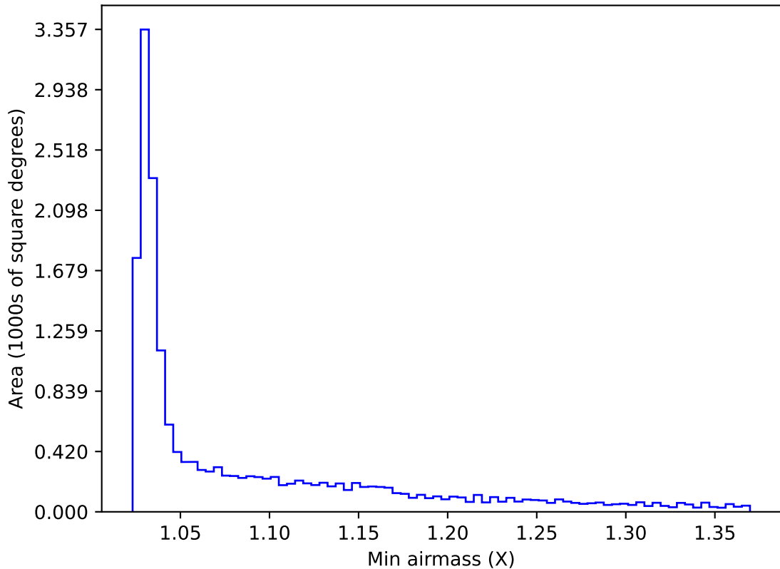
internal_u_expt27_nscale1.5v3.4_10yrs WFD y band: Min airmass
