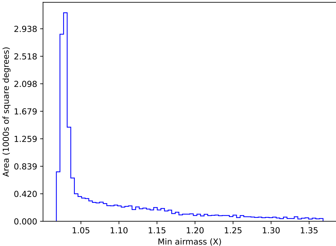
internal_u_expt27_nscale1.5v3.4_10yrs WFD i band: Min airmass
