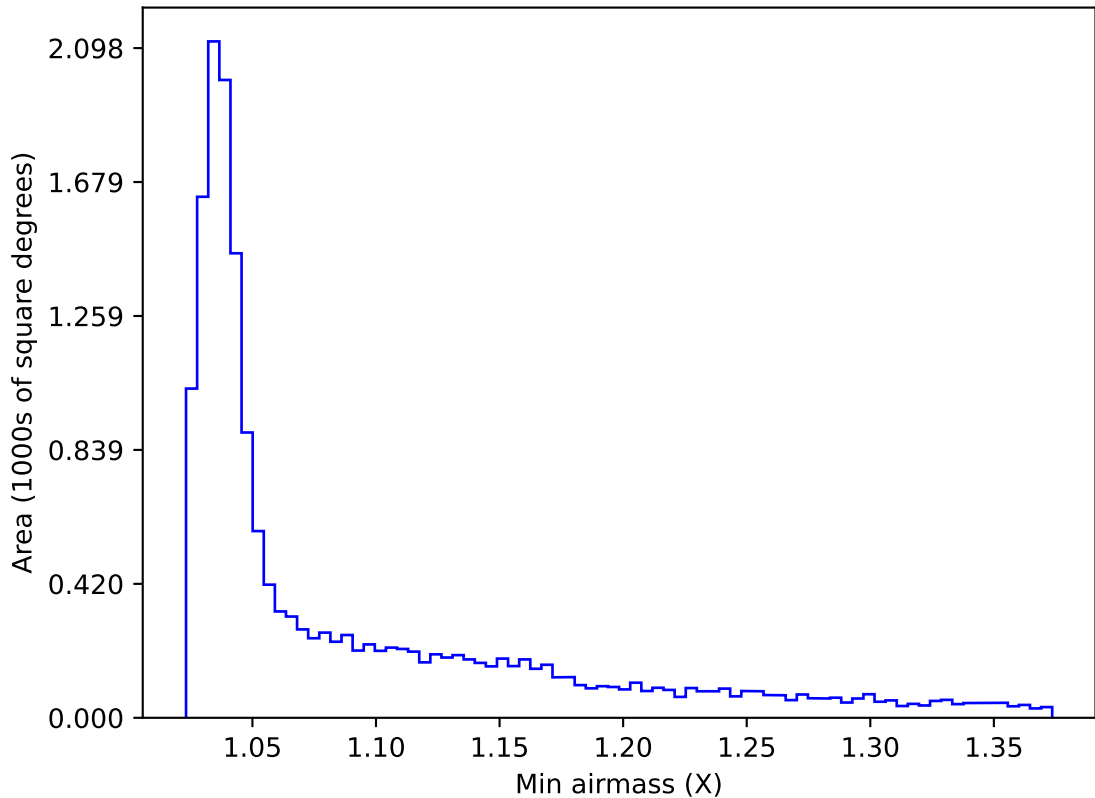
internal_u_expt27_nscale1.5v3.4_10yrs WFD g band: Min airmass
