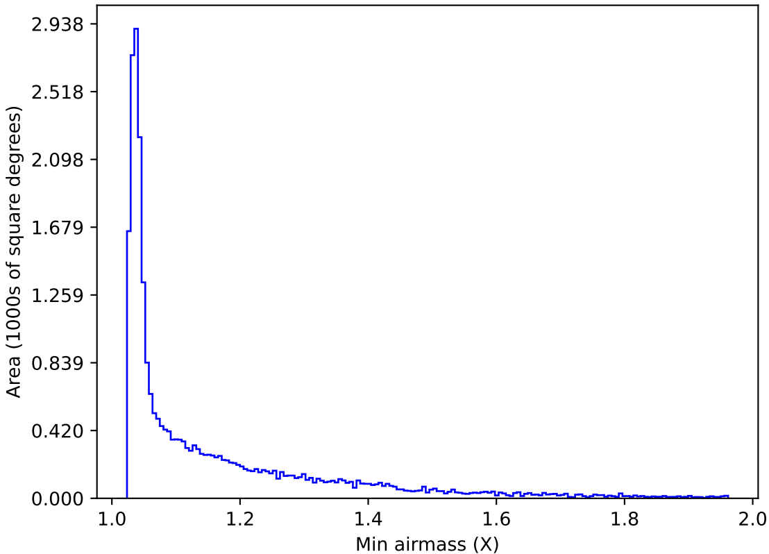
internal_u_expt27_nscale1.5v3.4_10yrs All sky g band: Min airmass
