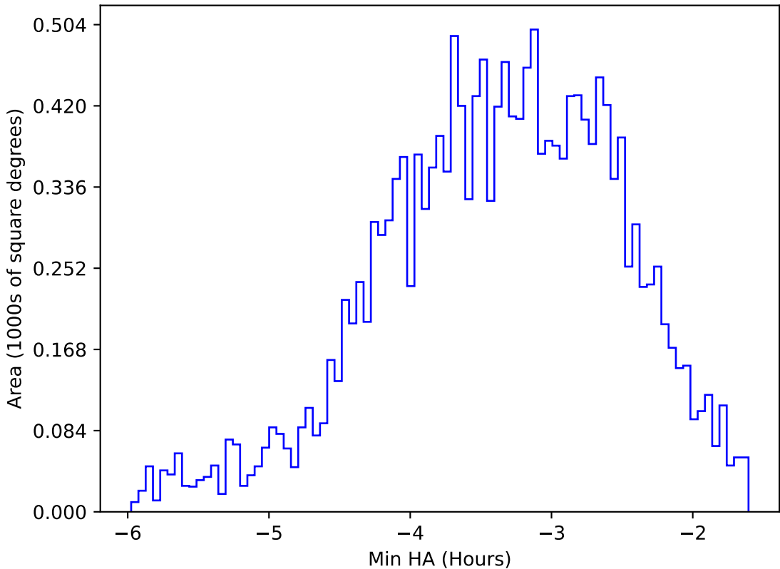
internal_u_expt27_nscale1.5v3.4_10yrs WFD u band: Min HA
