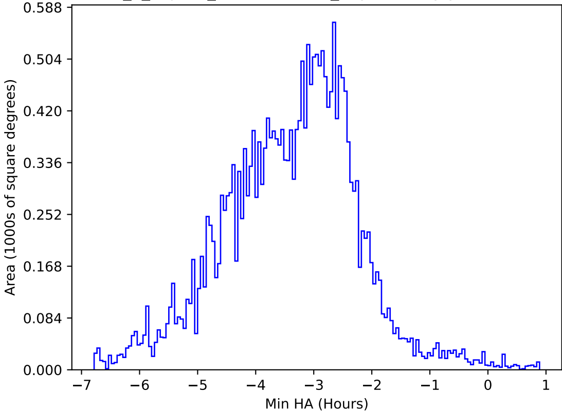
internal_u_expt27_nscale1.5v3.4_10yrs All sky y band: Min HA
