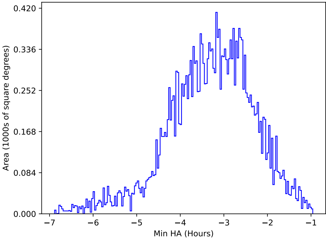
internal_u_expt27_nscale1.5v3.4_10yrs All sky u band: Min HA
