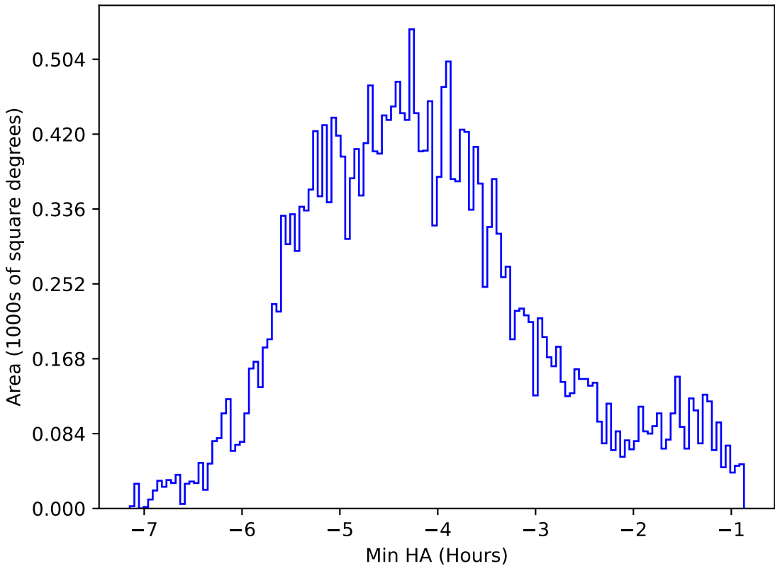
internal_u_expt27_nscale1.5v3.4_10yrs All sky r band: Min HA
