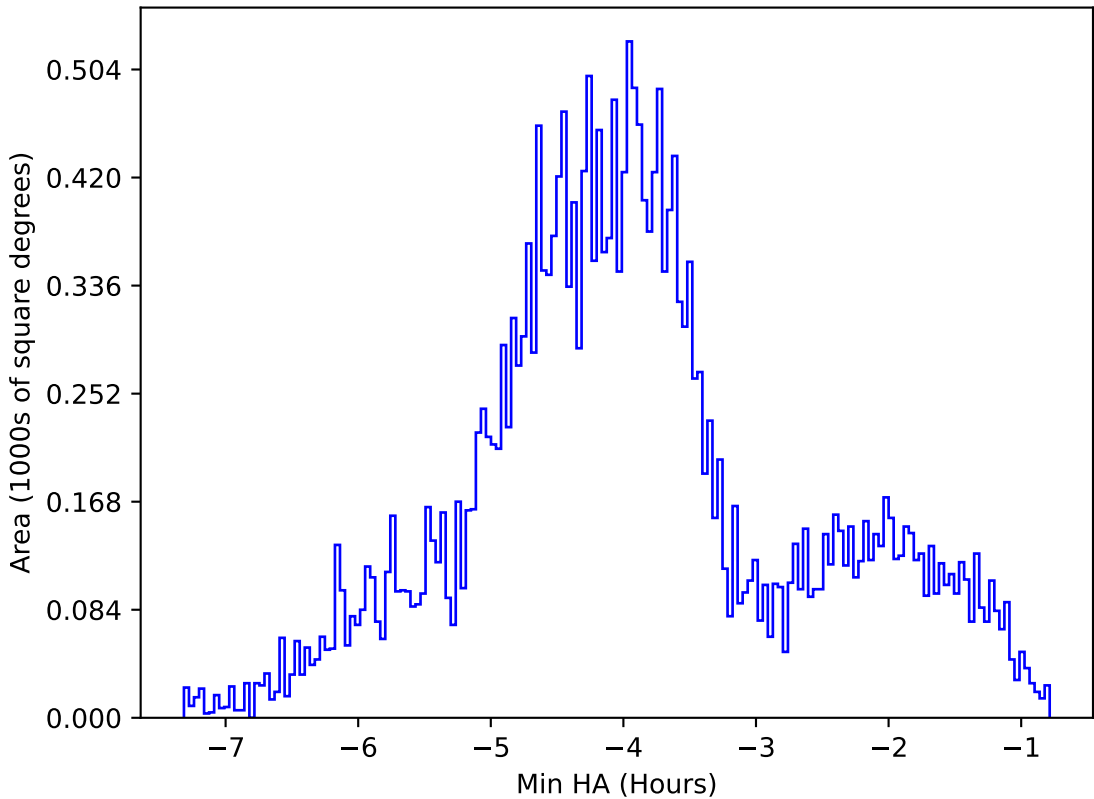
internal_u_expt27_nscale1.5v3.4_10yrs All sky g band: Min HA
