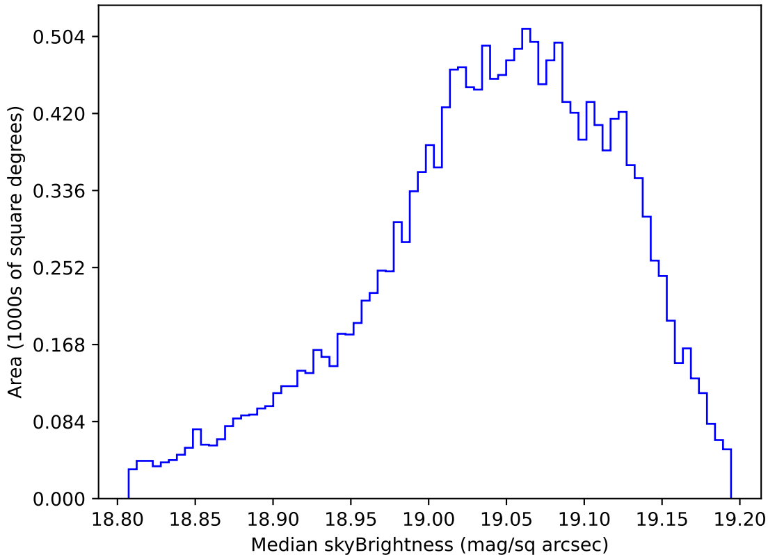
internal_u_expt27_nscale1.5v3.4_10yrs WFD z band: Median skyBrightness
