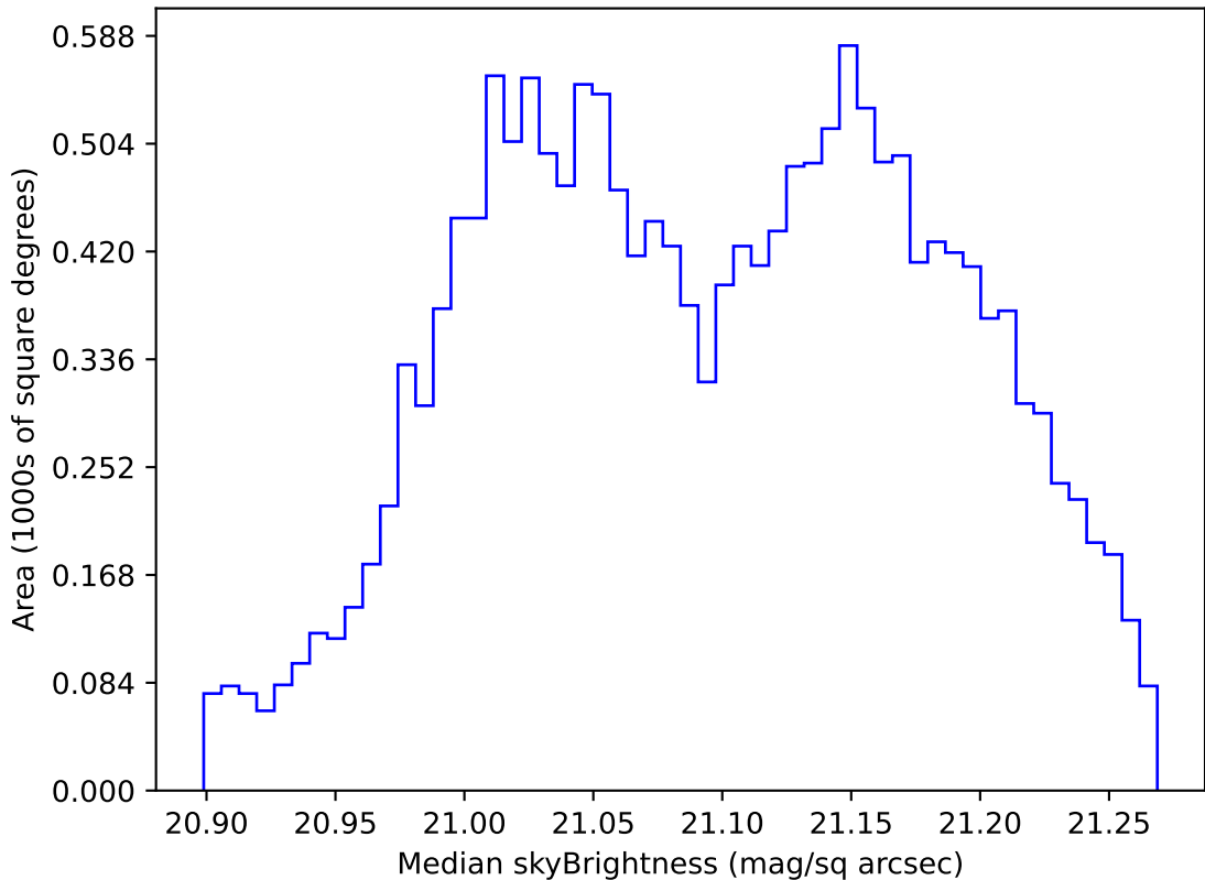
internal_u_expt27_nscale1.5v3.4_10yrs WFD r band: Median skyBrightness
