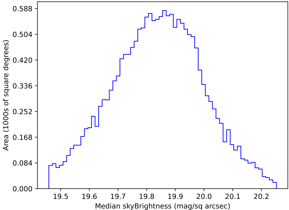
internal_u_expt27_nscale1.5v3.4_10yrs WFD all bands: Median skyBrightness
