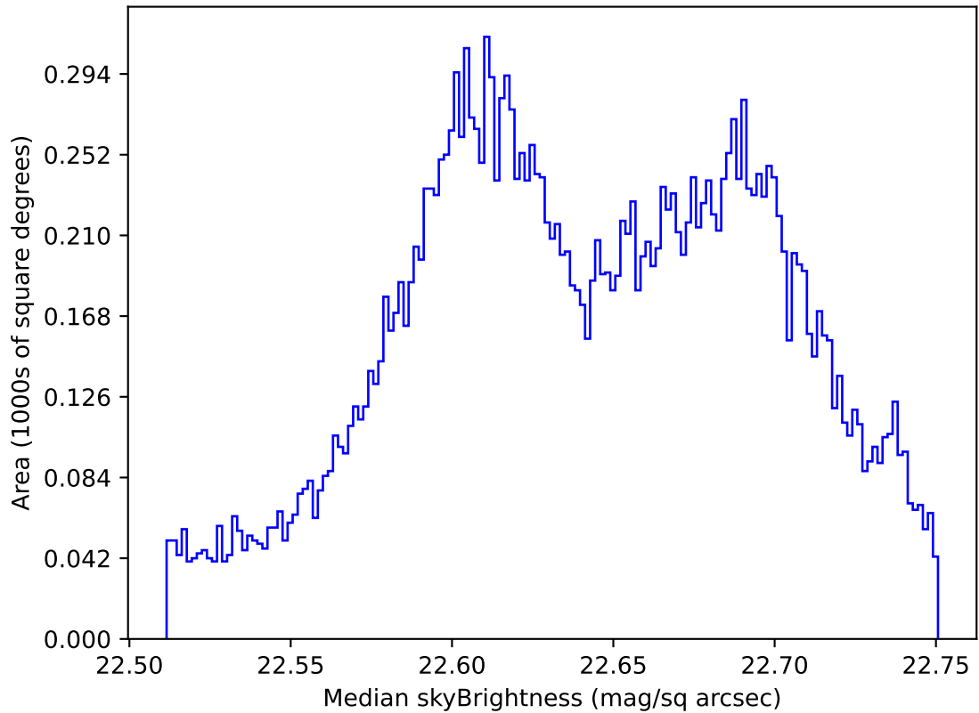
internal_u_expt27_nscale1.5v3.4_10yrs All sky u band: Median skyBrightness
