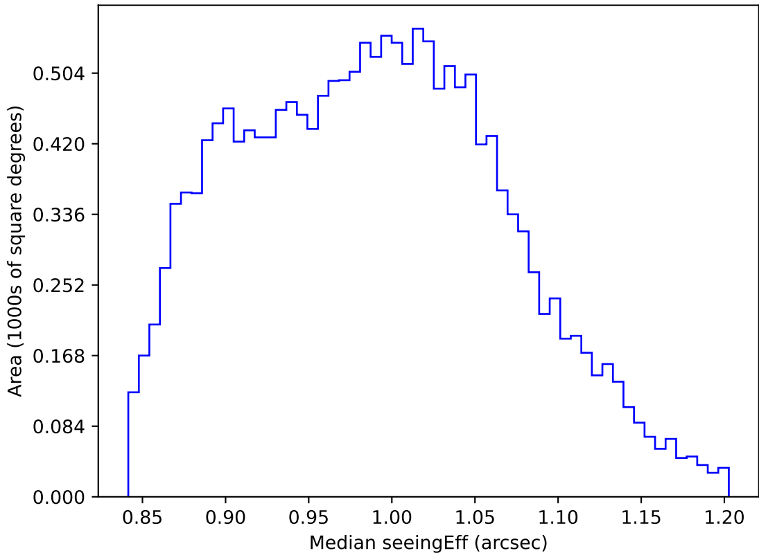
internal_u_expt27_nscale1.5v3.4_10yrs WFD i band: Median seeingEff
