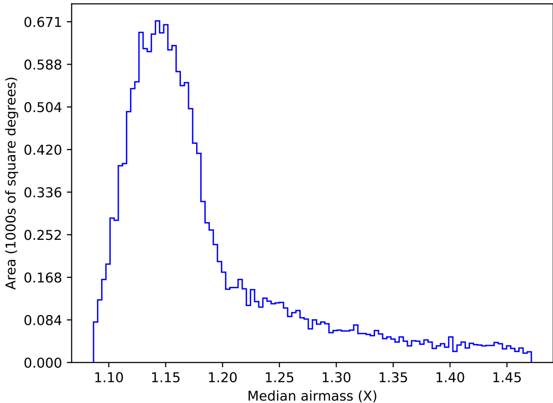
internal_u_expt27_nscale1.5v3.4_10yrs WFD z band: Median airmass
