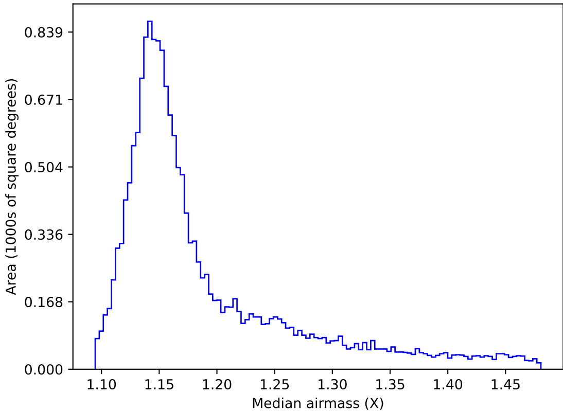
internal_u_expt27_nscale1.5v3.4_10yrs WFD y band: Median airmass
