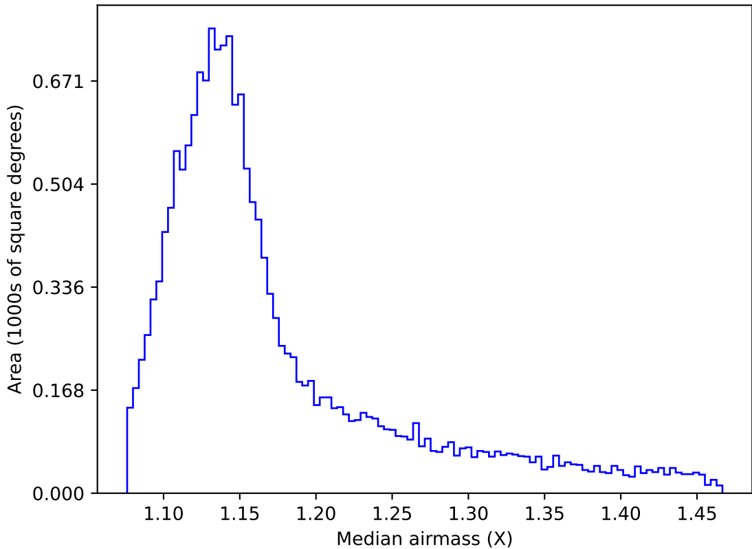
internal_u_expt27_nscale1.5v3.4_10yrs WFD r band: Median airmass
