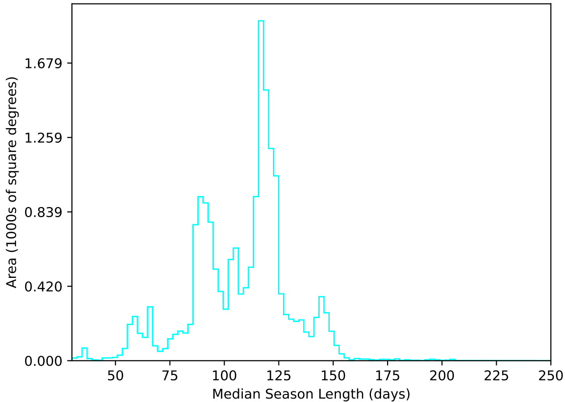
internal_u_expt27_nscale1.5v3.4_10yrs WFD u band: Median Season Length
