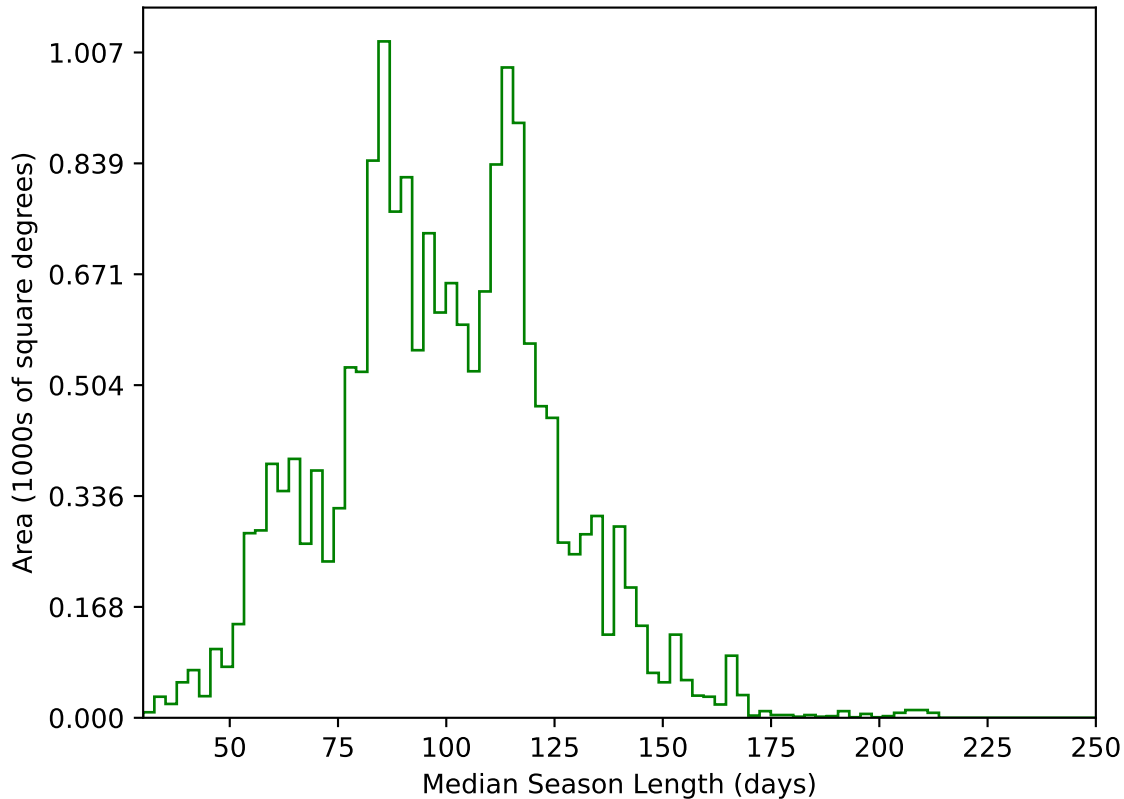
internal_u_expt27_nscale1.5v3.4_10yrs WFD g band: Median Season Length
