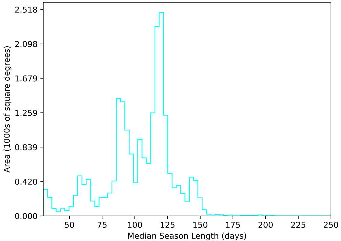
internal_u_expt27_nscale1.5v3.4_10yrs All sky u band: Median Season Length
