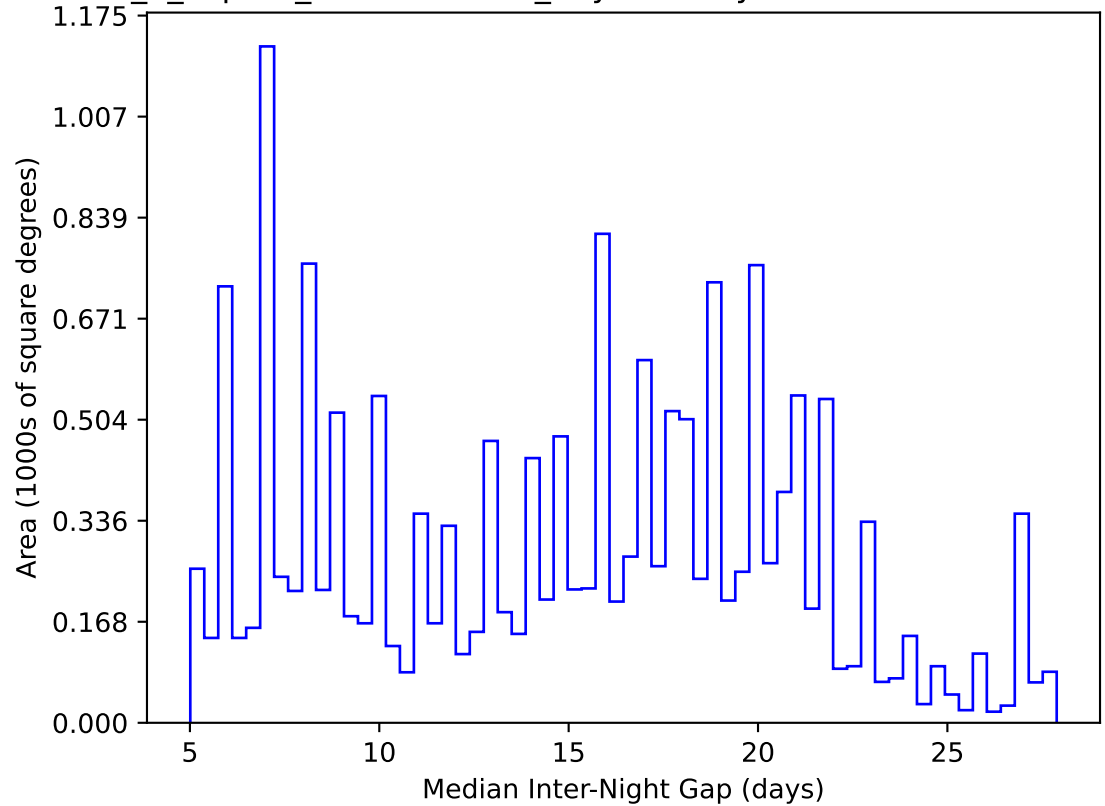
internal_u_expt27_nscale1.5v3.4_10yrs WFD y band: Median Inter-Night Gap
