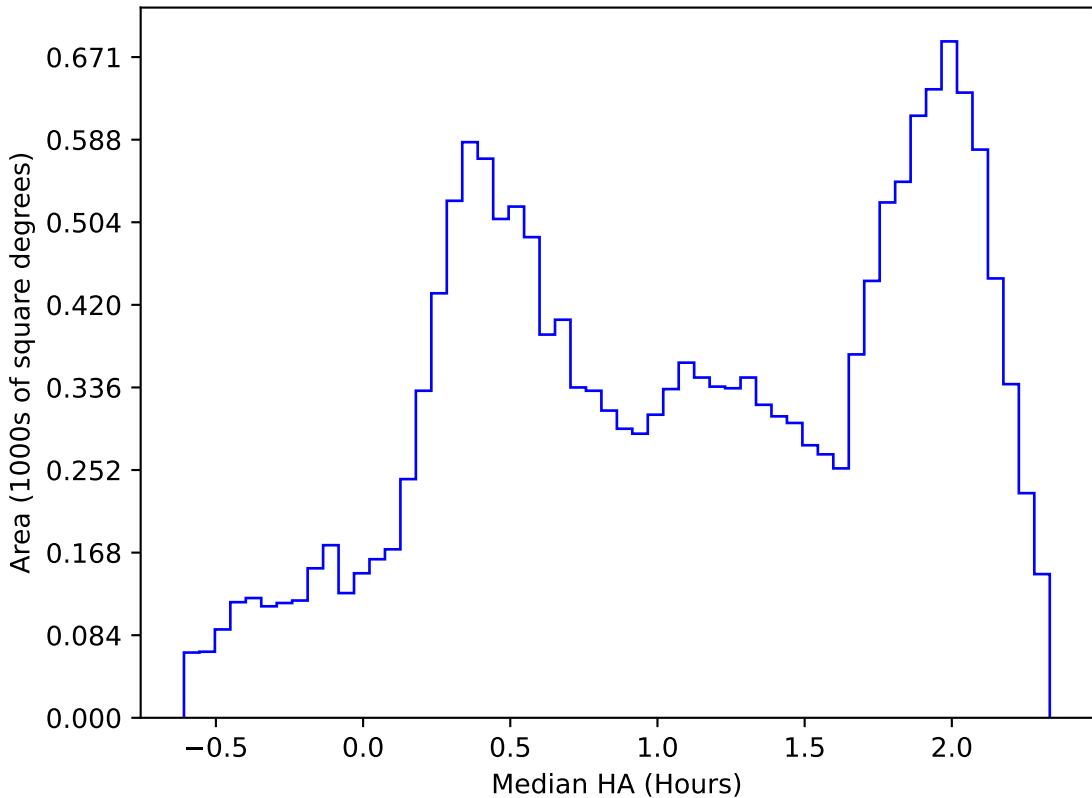
internal_u_expt27_nscale1.5v3.4_10yrs WFD z band: Median HA
