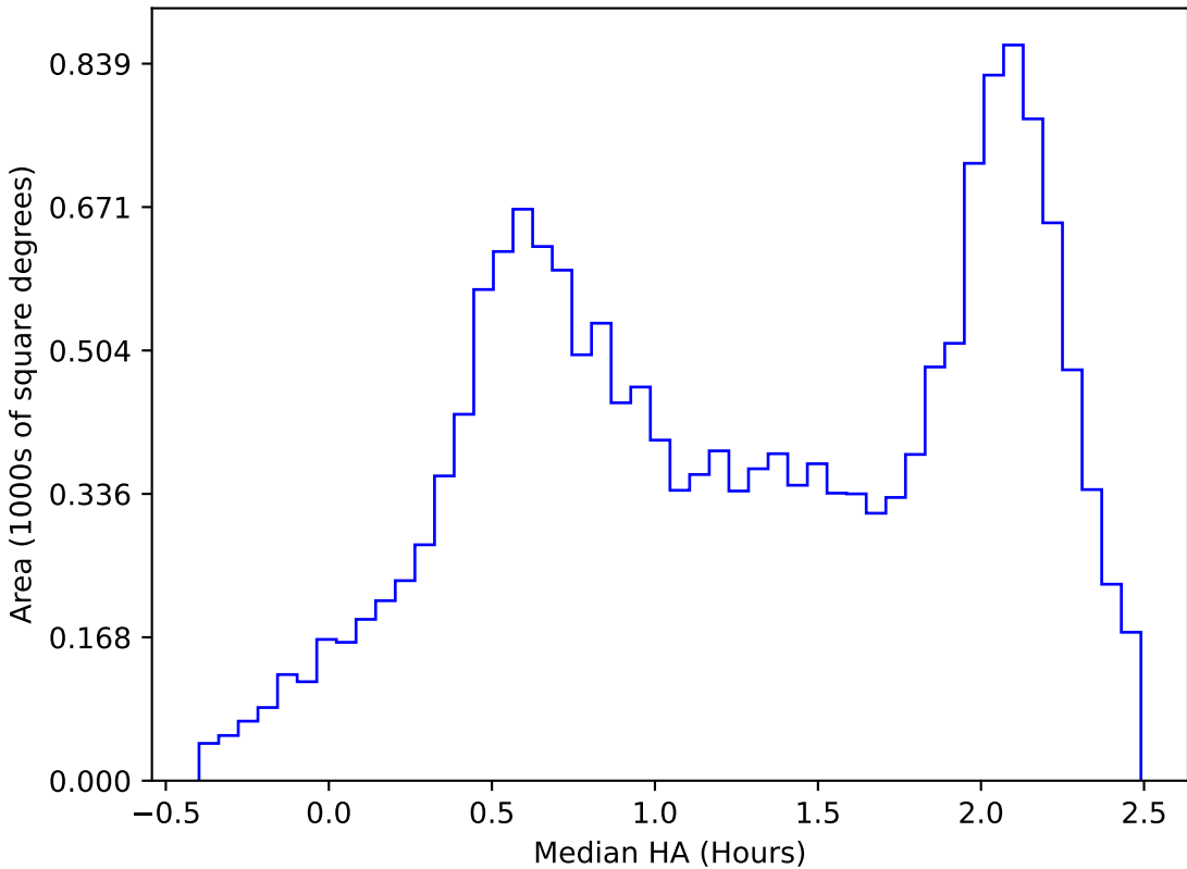
internal_u_expt27_nscale1.5v3.4_10yrs WFD y band: Median HA
