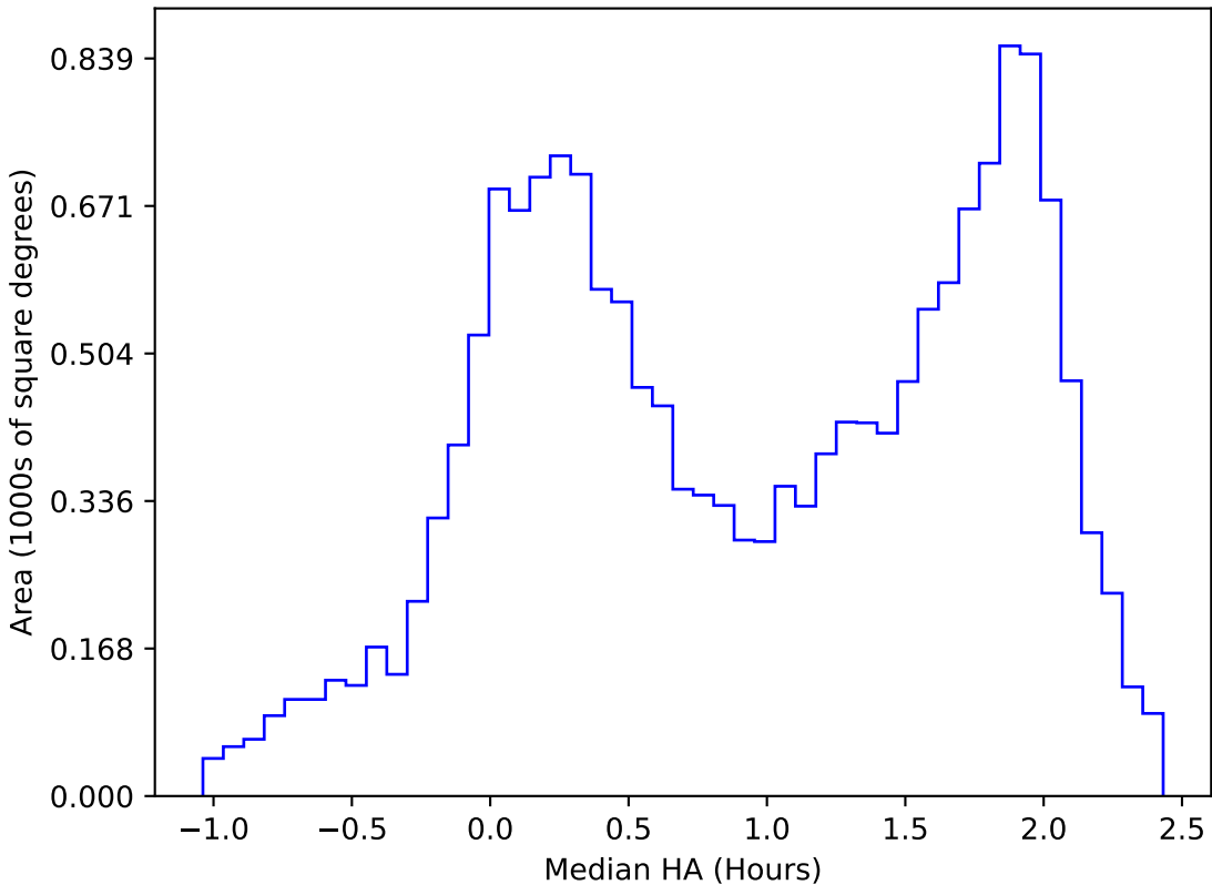
internal_u_expt27_nscale1.5v3.4_10yrs WFD u band: Median HA
