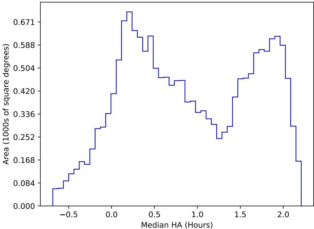
internal_u_expt27_nscale1.5v3.4_10yrs WFD r band: Median HA
